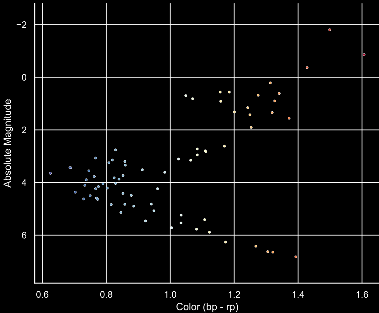
GALAH Hertzprung-Russel Diagram Field [96] Ra [333.02] Dec [-67.63]
