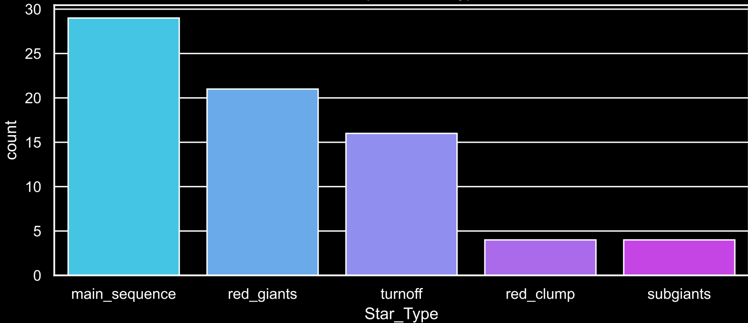
Field [96] Count plot of Star Type
