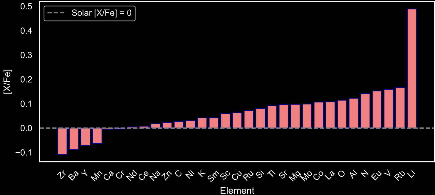
Abundance Pattern for GALAH Star Field [96] (N=74)
