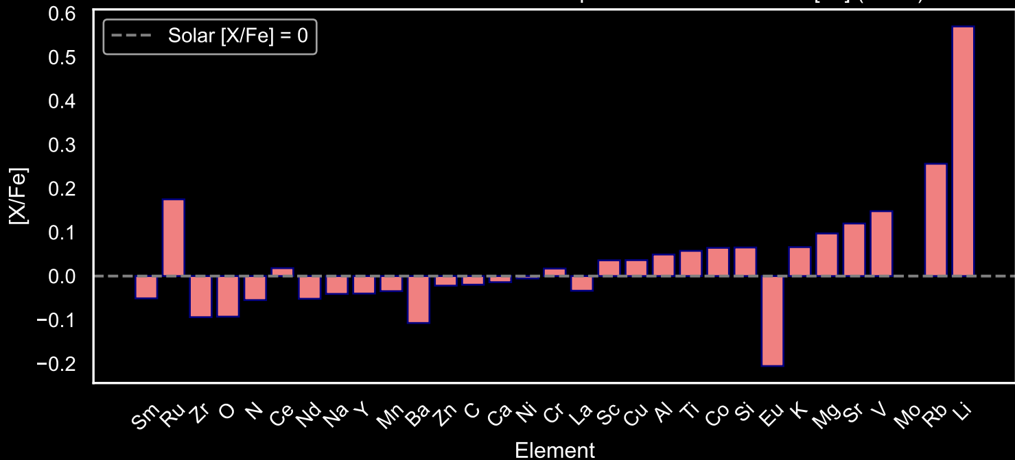
Abundance Pattern for GALAH Main Sequence Stars: Star Field [96] (N=29)
