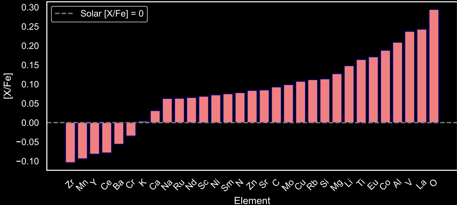
Abundance Pattern for GALAH Red Giants: Star Field [96] (N=25)
